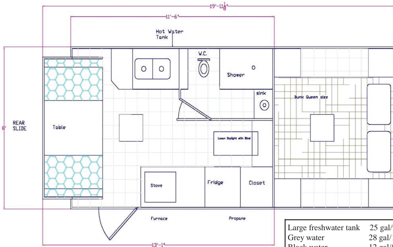
MOTOR HOME FLOOR PLAN
